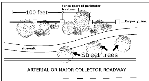
Figure 24-25: Perimeter Treatment for Residential and Institutional Next to Major Collector or Arterial Roadway
