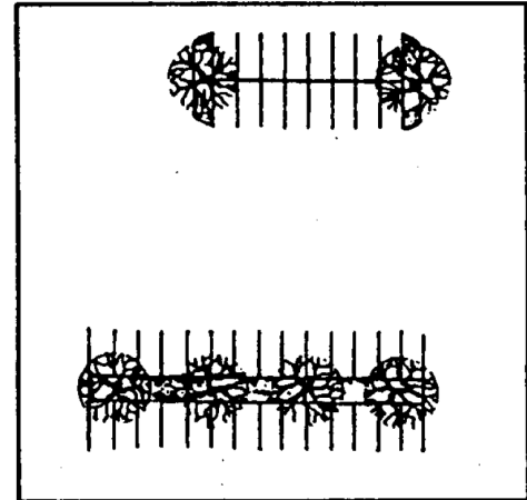
Figure 24-24: Parking Lot Islands (Top) and Medians (Bottom)
