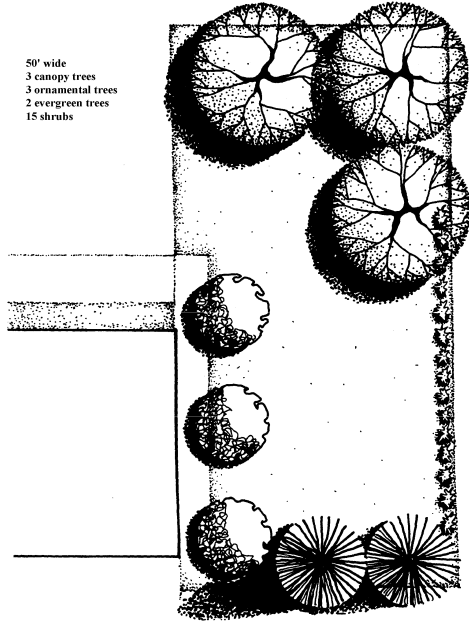
Figure 24-22: Buffer Yard "E"
