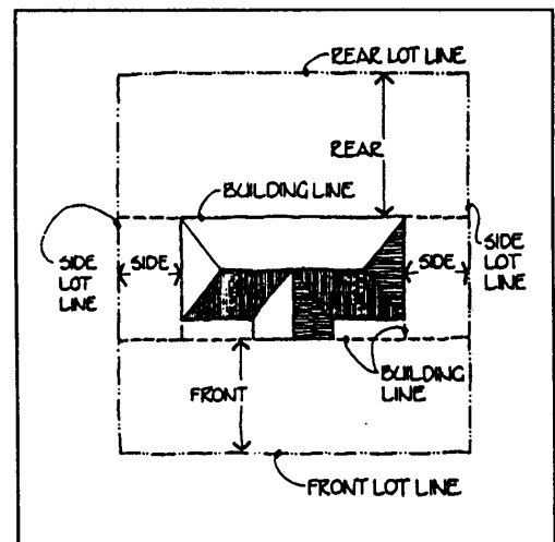
Figure 24-2: Buildable Area Defined by Setbacks
