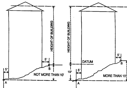
Building Height from Ground
