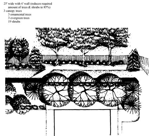
Figure 24-21: Buffer Yard "D"
