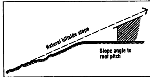
Figure 24-36: Roof Pitch Reflects Hillside Slope
