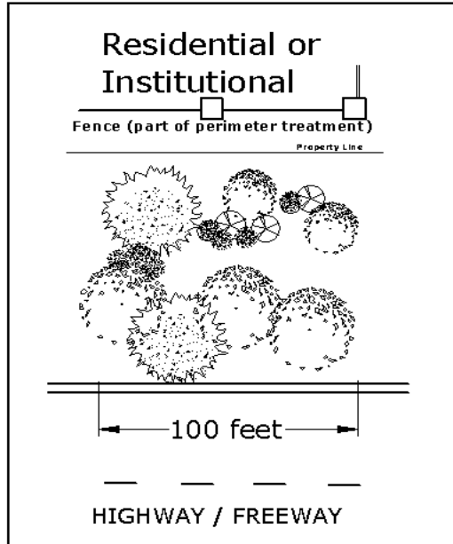
Figure 24-26: Perimeter Treatment for Residential and Institutional Next to Highway, Freeway or Expressway
