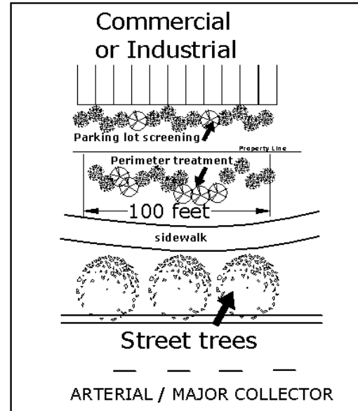
Figure 24-26.1: Perimeter Treatment for Commercial and Industrial Next to Major Collector or Arterial Roadway
